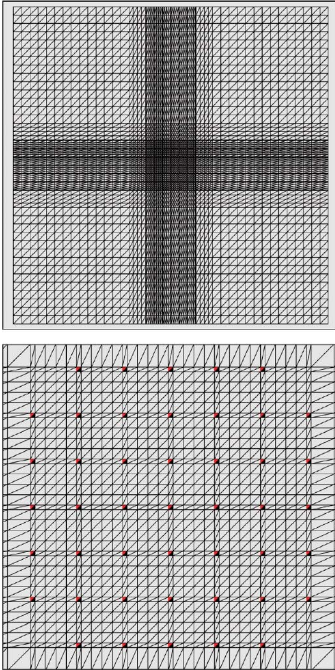
Figure 2-1. Horizontal sections showing the discretisation of the model grid. The top picture shows the entire model domain and the bottom picture is a close-up view over the central part of the grid containing the 45 boreholes (red markers). (The triangles are an artefact of the program used to plot the grid.)
