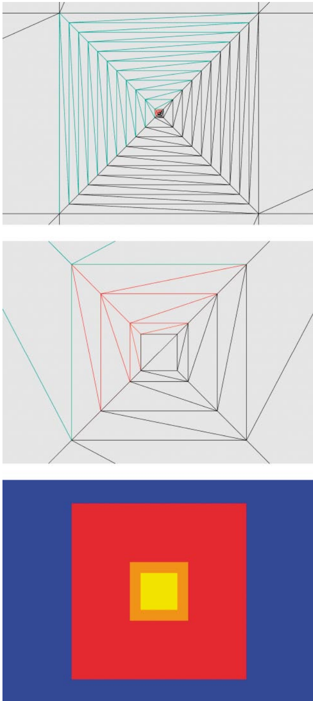
Figure 2-5. Close-up view of a horizontal section through one single borehole showing the azimuthal discretisation, borehole materials and rock type. (The triangles are an artefact of the program used to plot the grid.)
