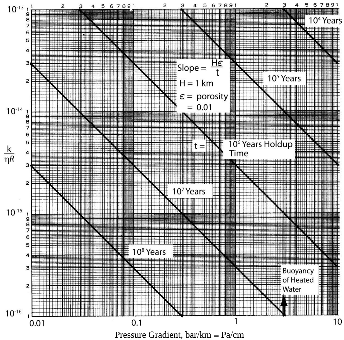
Fig. 1. Transport delay provided by 1 km caprock.
