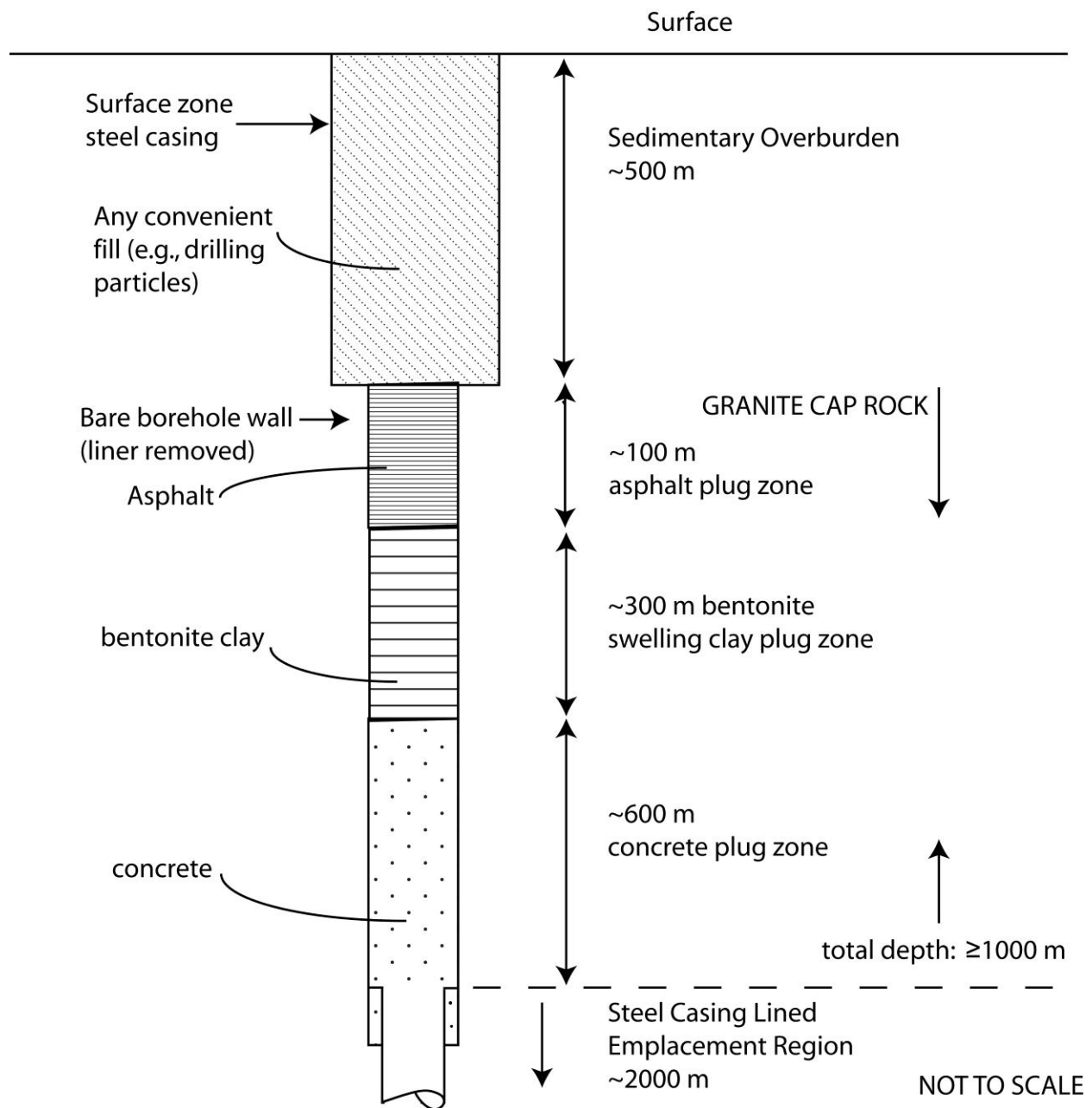
Fig. 4. Schematic of Borehole Plug Design Features.
