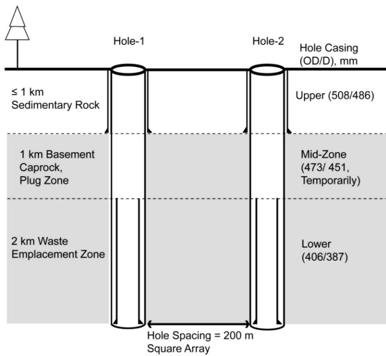
Fig. 3. Deep Borehole HLW Disposal Concept.
